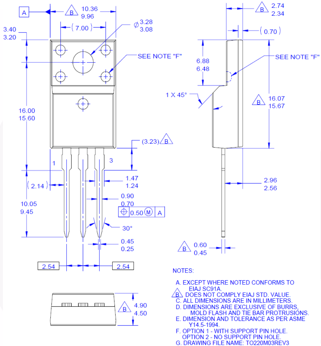
Figure 19. TO-220F 3L - TO220, MOLDED, 3LD, FULL PACK, EIAJ SC91, STRAIGHT LEAD
